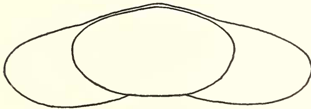
B TEXT-FIG. 7. Alisporites toralis comb. nov. Diagrammatic reconstructions. A, Polar view. B, Polar section. \times 1,000 .
